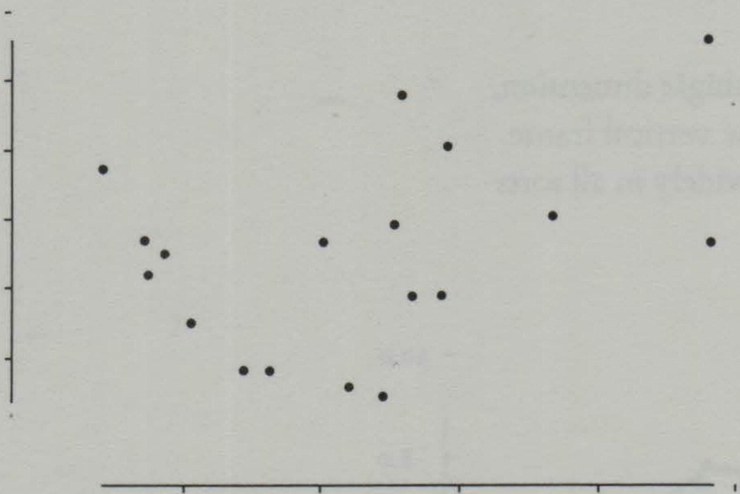
Range-Frame
