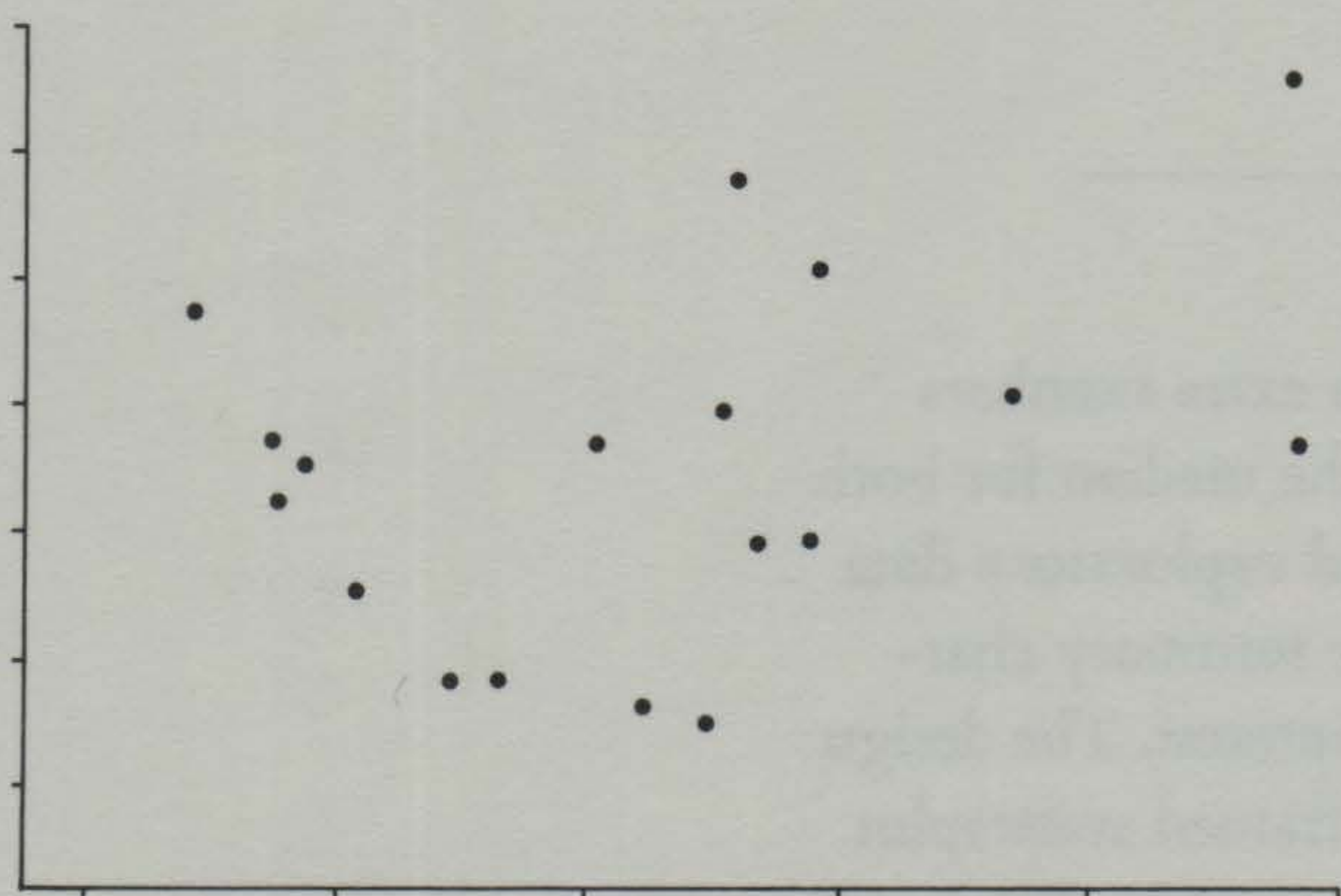
Conventional Scatterplot
